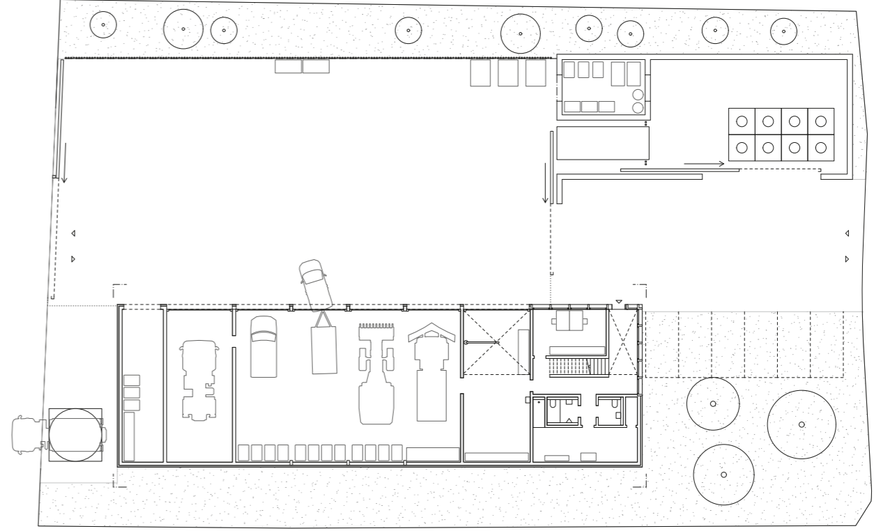
erdgeschoss · ground floor
